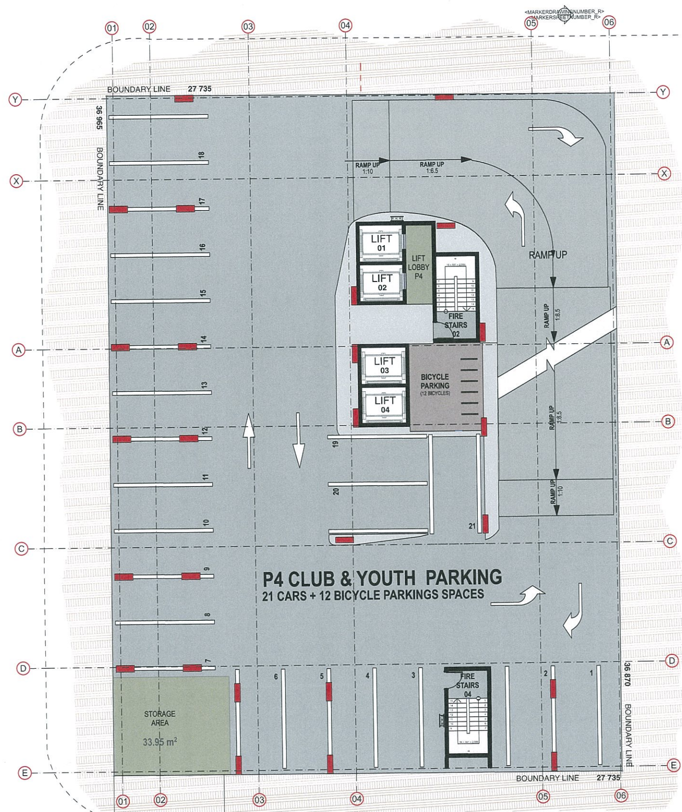
1 P4 CLUB + YOUTH CENTRE PARKING
