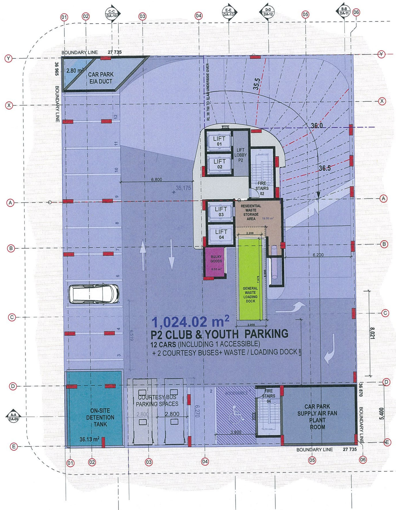
1 P2 CLUB + YOUTH CENTRE PARKING
