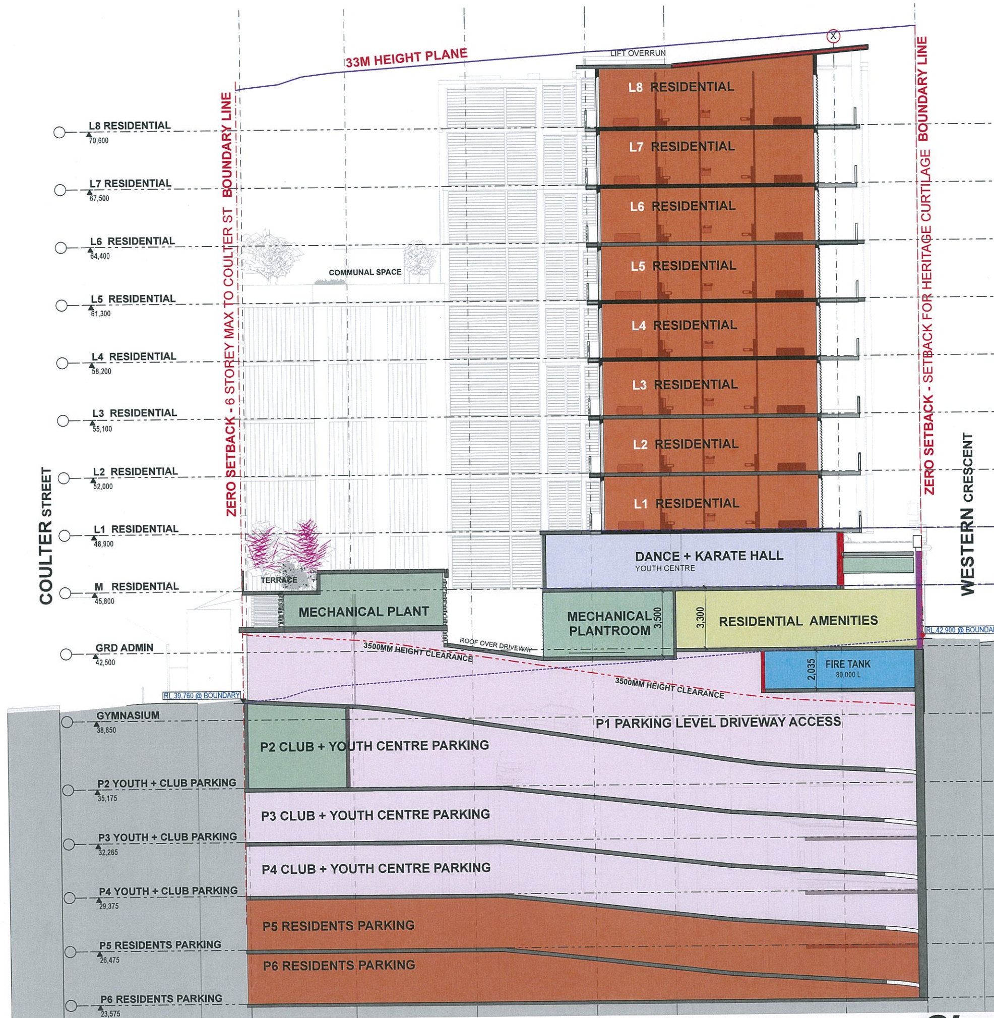
LONG SECTION THRU DANCE + KARATE (B-B)
