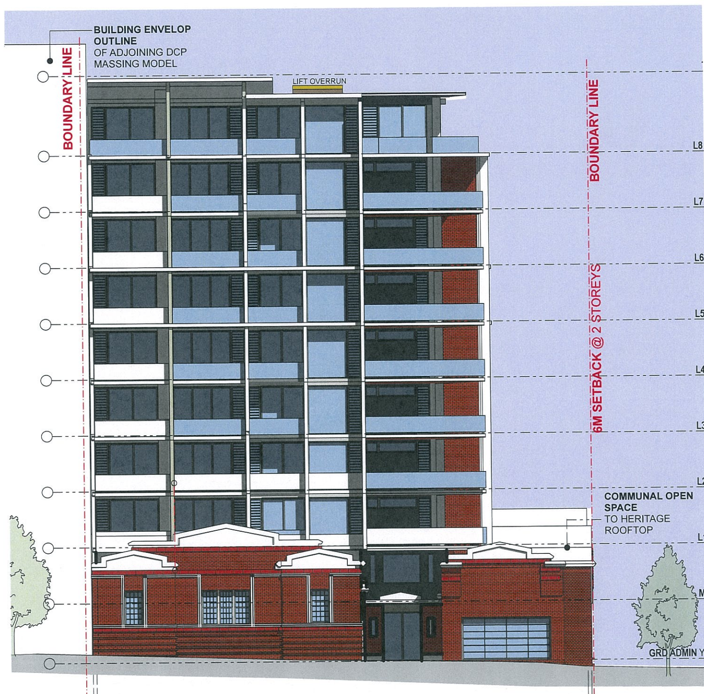
1 EAST ELEVATION (WESTERN CRESCENT)
