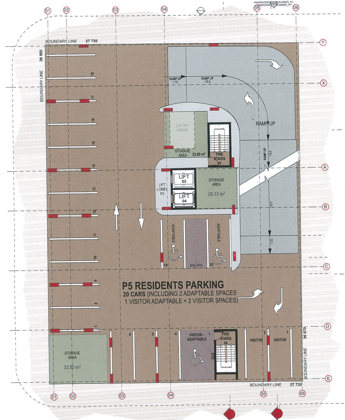
1 P6 RESIDENTS PARKING
