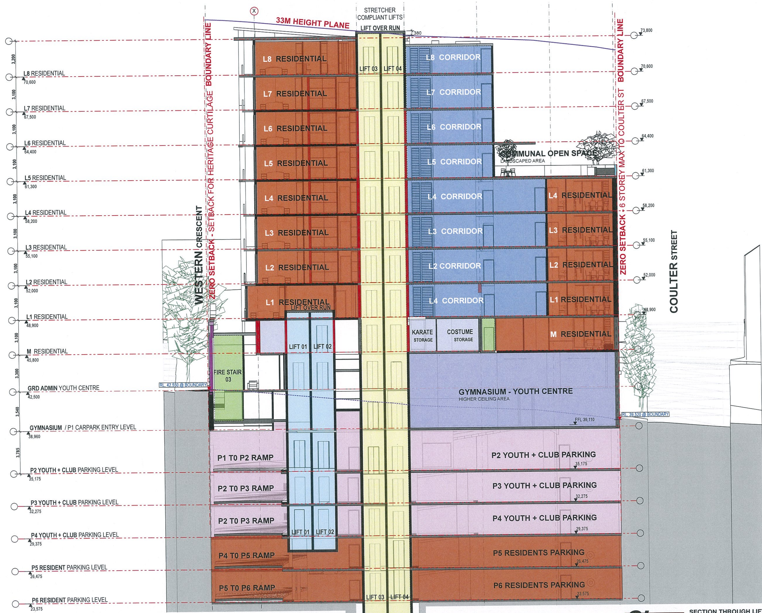
SECTION THROUGH LIFTS (E-E)
