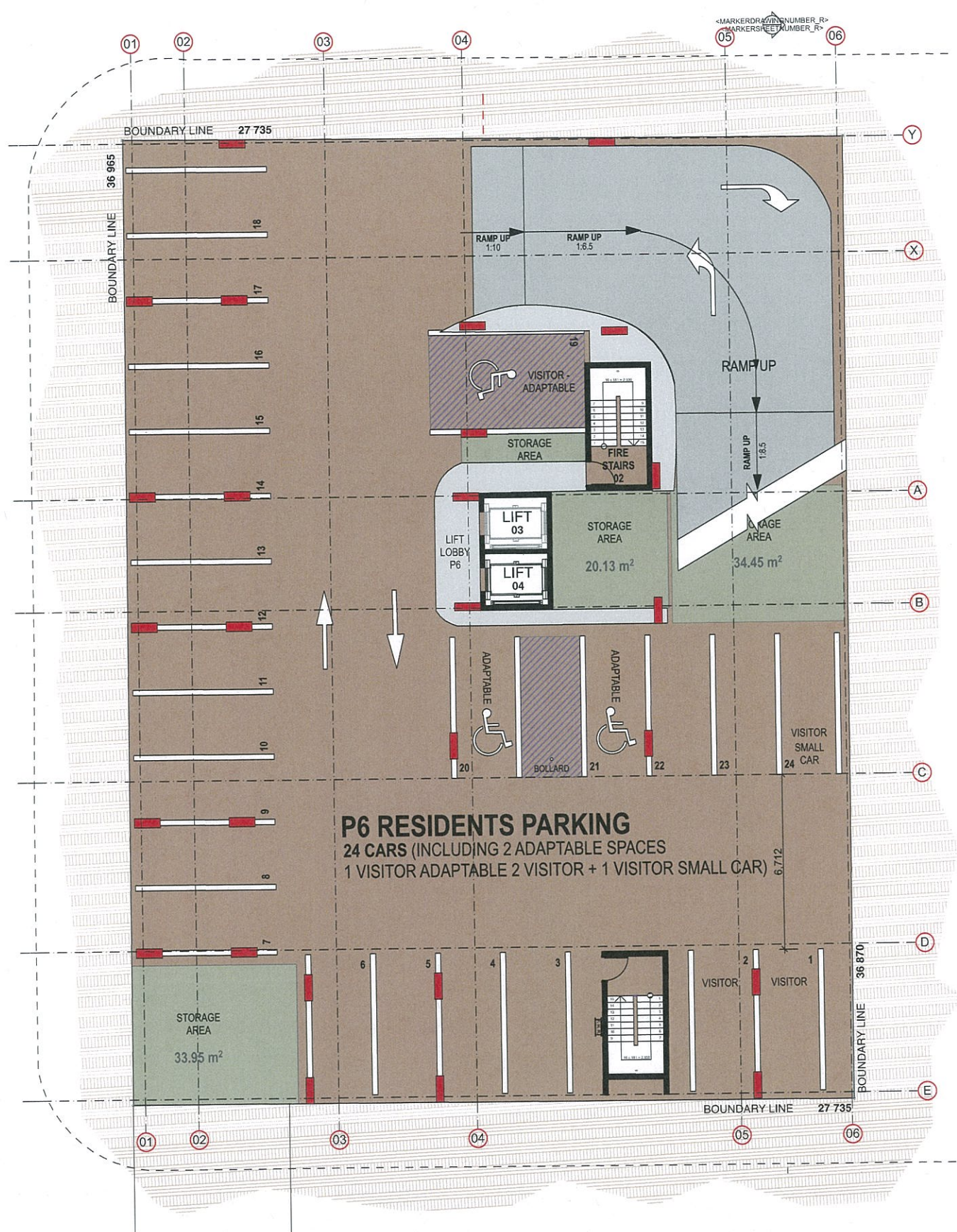
2 P6 RESIDENTS PARKING
